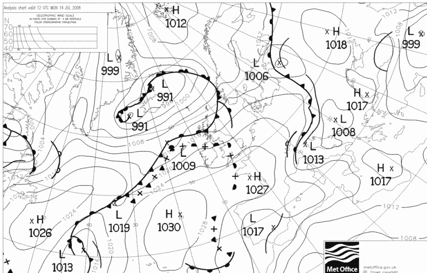
Fig. 1. Field of atmospheric pressure at ground level over Europe, on July 14 th 2008, 12 00 UTC (according to www.wetterzentrale.de ).
