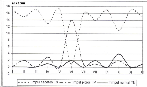
Figure No 4. The evolution of drought in 1992 in rates of number of cases on time types in conformity with Hellmann's Criterion.
