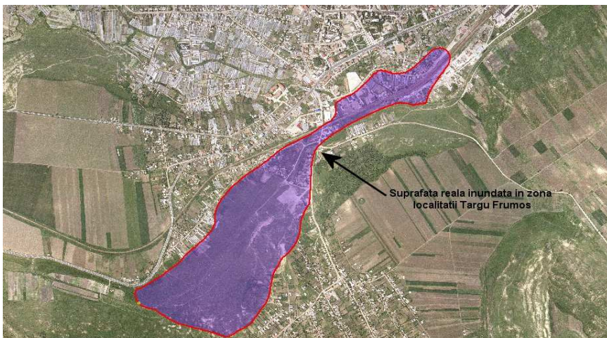
Fig. 8. The real surface flooded near Târgu Frumos after the flood from the night of July 24-25, 2008
