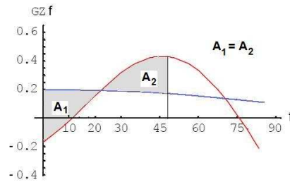
Fig. 8. Graphical estimation of the maximum dynamical heeling angle of approx. 47^\circ (Chiotoroiu L., 2007)
