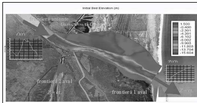
Fig. 2. The conditions at the limit specified on the upstream and downstream frontiers of the hydrodynamic model for the calculations done in a permanent and non-permanent regime
