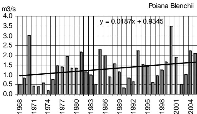
Fig. 3. Poiana Blenchii hydrometric station spring runoff trend
