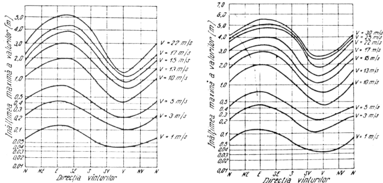
Fig. 2. Wave's height vs. wind speed and direction: Sulina, 15 m depth (on the left) and Constanta, 9 m depth (on the right), Bondar (coord.), 1972.
