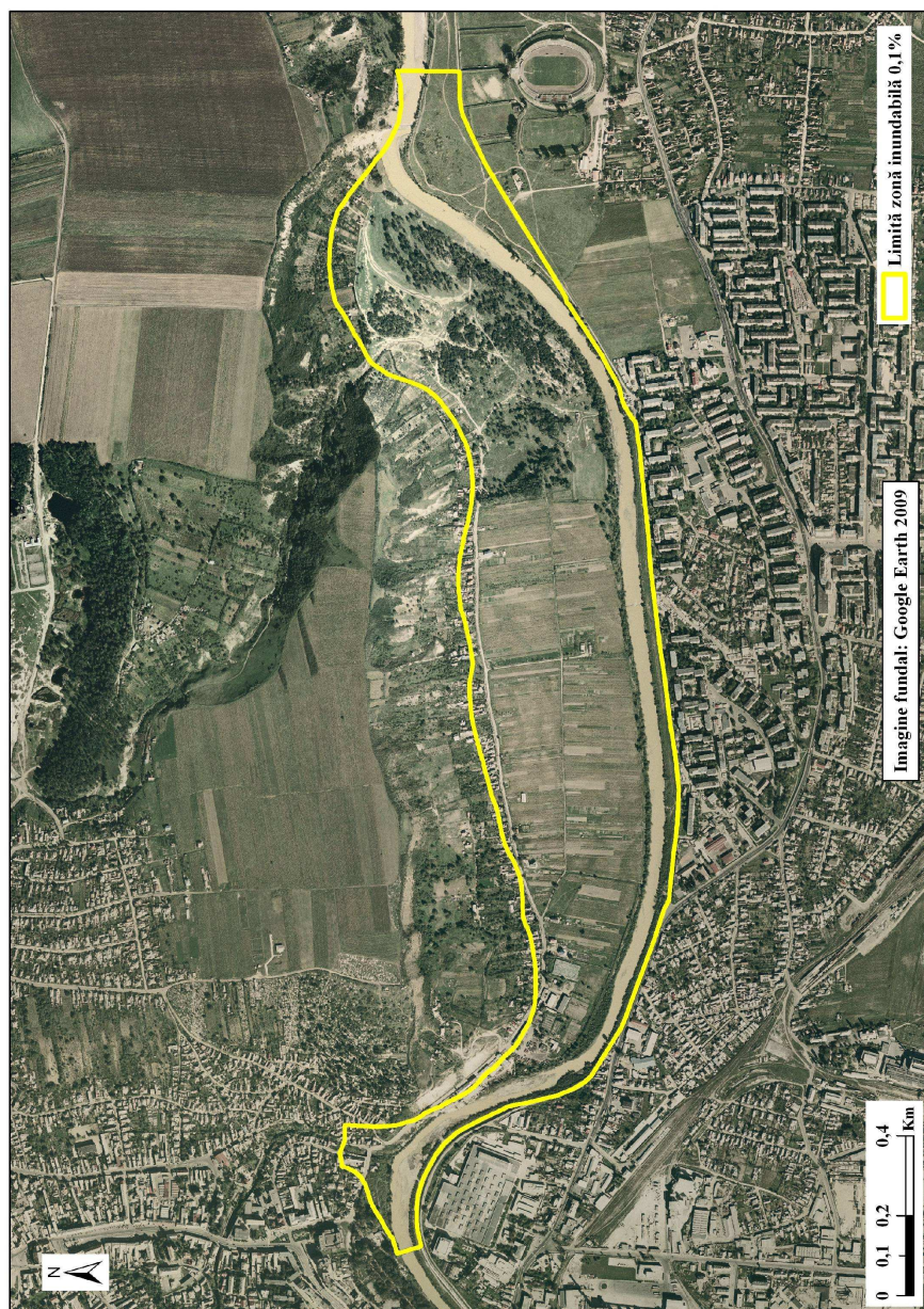
Fig. 4. The flooded area related to the non-exceedence probability of 0.1 % on the Arieș Valley at Turda
