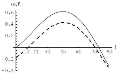
Fig. 7. Effect on the curve of statical stability of static list of approx. 11^\circ (Chiotoroiu L., 2007)
