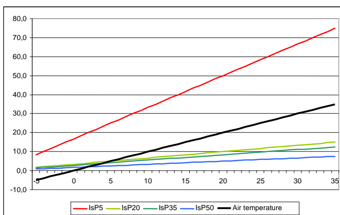
Fig. 2. The variation in intensity of a ten days interval lacking precipitations according to air temperature, in the conditions of standard precipitation values for the previous decade
