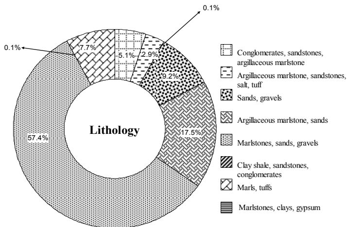
Fig. 2. Distribution of deep-seated landslides from Transylvanian Basin depending on the lithology.
