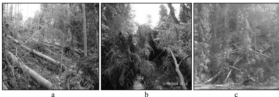
Fig. 4. a, b, c. Windthrows in June 2010 in Isticeu Valley.
