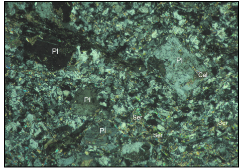
Fig. 4. The microscopical image of monzodiorite porphyric (N+), Pl-plagioclase, Cal-calcite, Ser-sericite.
