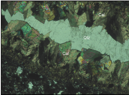
Fig. 3. The microscopical image of graywacke with calcite vein (N+), Qtz-quartz, Cal-calcite.
