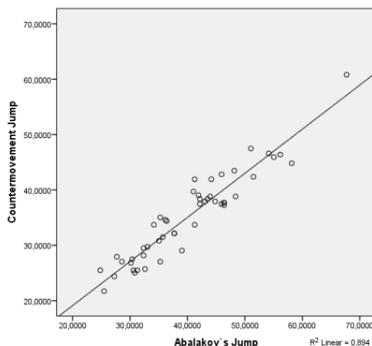
Fig. 6. Pearson correlation graph between Countermovement Jump and Abalakov's Jump (explosive power - boys)
