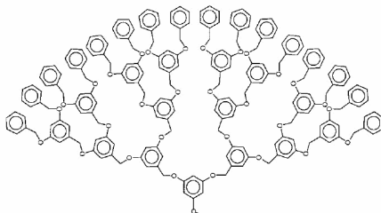
Figure 2. A dendritic wedge, of generation r=4 ; v=248 ; e=278 .
