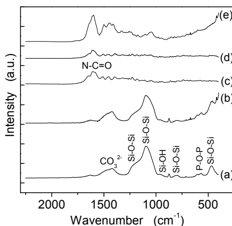
Figure 4. FT-IR spectra of glass (a), glass immersed in SBF (b), tetracycline (c), glass with tetracycline (d) and of glass after 96 hours immersion in SBF for tetracycline release (e).
