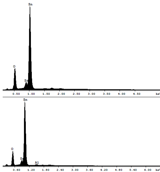
Figure 1. EDAX analysis of ZnO and AZO thin films (d=8cm for both samples)
