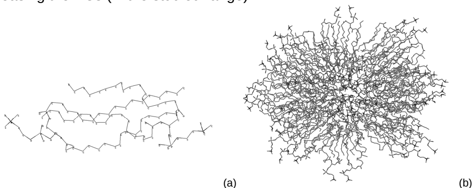
Figure 1. The most stable assemblies of the liposome PC unit, 2×PC (a) and the optimized smaller unilamellar liposome consists of 96 PC units (b)
