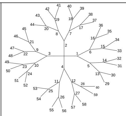
Figure 2. The Forth Generation of Dendrimer Molecule D_2[4] .
