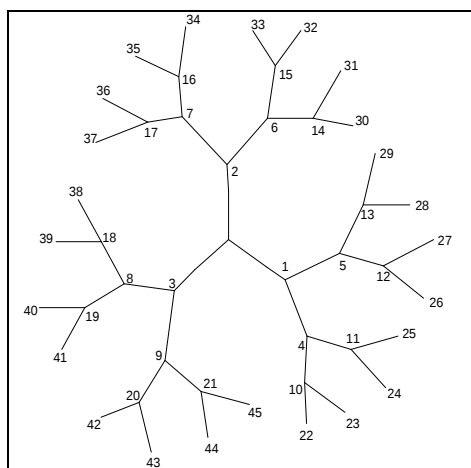
Figure 1. The Forth Generation of Dendrimer Molecule D_1[4] .
