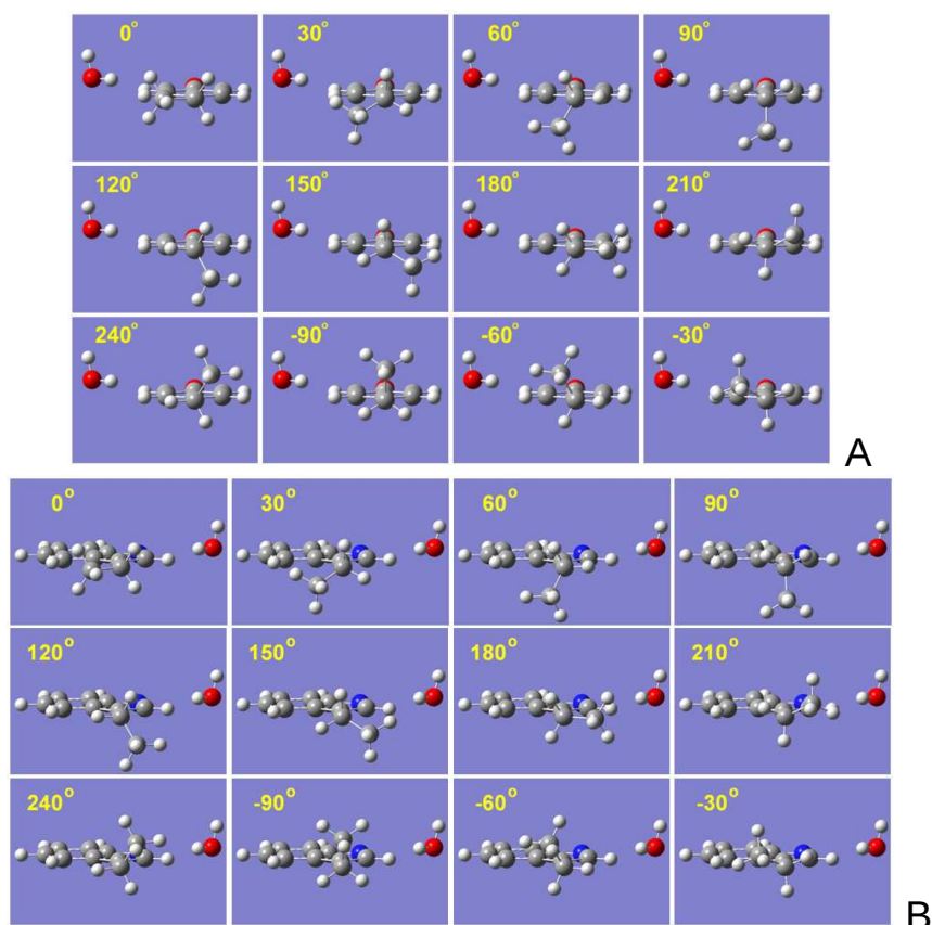
Figure 2. Twelve rotational conformations of the phenoxyl ring (plus water, d = 4.20 Å) in tyrosyl radical (A) and twelve rotational conformations of the indole ring (plus water, d = 4.20 Å) in tryptophanyl radical (B). The values of the dihedral angle \phi_6 = C\alpha-C\beta-C1-C6 (in Tyr, A) and \phi_4 = C\alpha-C\beta-C3-C4 (Trp, B) are shown on each pane.
