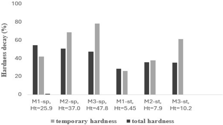
Figure 3. Decrease in temporary/total hardness of the blank samples after standing in the oven
