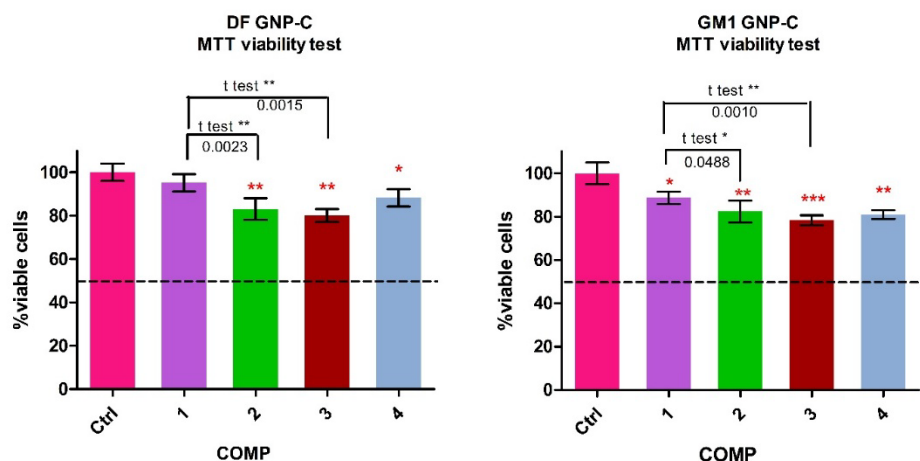
Figure 8: Cell viability (viable cells in % of Control, from MTT assay): Control (Ctrl); 1) GNP-C 3.9 \mu\text{g/mL} ; 2) GNP-C 3.9 \mu\text{g/mL} / P 0.67 \mu\text{g/mL} ; 3) GNP-C/A 3.9 \mu\text{g/mL} D 0.21 \mu\text{g/mL} ; 4) GNP-C 3.9 \mu\text{g/mL} / Ic 1.67 \mu\text{g/mL}
