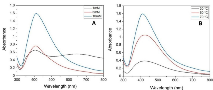
Figure 1. UV-Vis spectra: Effect of concentration and temperature on silver nanoparticles synthesis: (A) different concentrations of \text{AgNO}_3 , extract to \text{AgNO}_3 ratio = 1:20, T = 70\text{ }^\circ\text{C} , \text{pH} = 8 , reaction time = 4 h; (B) 10 mM \text{AgNO}_3 , extract to \text{AgNO}_3 ratio = 1:20, \text{pH} = 8 at different temperatures
