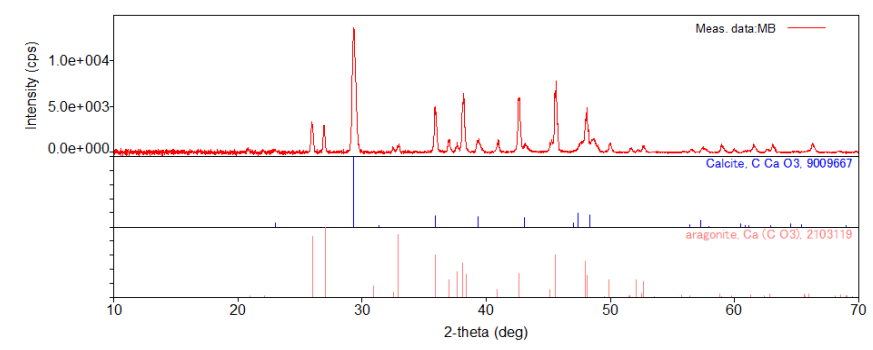
Figure 5a. X-ray diffractogram of \text{CaCO}_3 formed from the water sample with initial total hardness 25.9 mval/L
