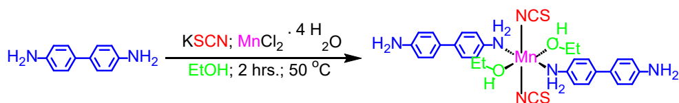
Scheme 1. Synthesis of \text{Mn}(4,4'\text{-DABPh})_2(\text{NCS})_2(\text{EtOH})_2 .
