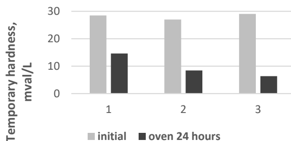
Figure 2a. Variation of temporary hardness in sparkling water blank samples 1 – H_t = 25.9 mval/L; 2 – H_t = 37 mval/L; 3 – H_t = 47.8 mval/L
