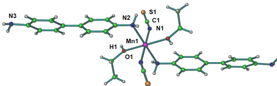
Figure 1. The molecular structure of the \text{Mn}(4,4'\text{-DABPh})_2(\text{NCS})_2(\text{EtOH})_2 complex.
