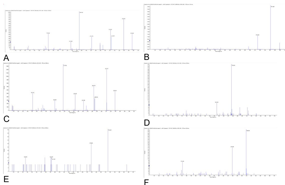
Figure 1. MS spectrum of compounds: A - CBDA, B - CBGA, C - CBVA, D - CBD, E - CBG, F – CBN
