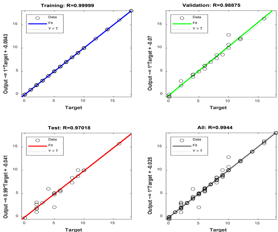
Figure 6. Actual concentrations versus the predicted concentrations and R values for training, validation, and testing series of the proposed ANN model
