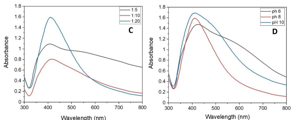
Figure 2. UV-Vis spectra: Effect of extract to \text{AgNO}_3 ratio and effect of pH on silver nanoparticles synthesis: (C) different extract to \text{AgNO}_3 ratio, 10 mM \text{AgNO}_3 , pH = 8, T = 70 °C, reaction time = 4 h; (D) extract to \text{AgNO}_3 ratio = 1:20, 10 mM \text{AgNO}_3 , T = 70 °C, reaction time = 4 h at different pH values
