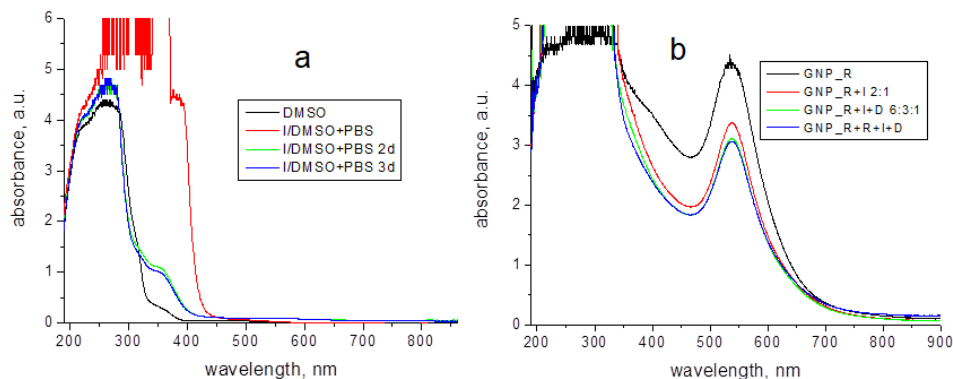
Fig. 6. UV-Vis spectra of DMSO, and of icariin (I, 100 mg/L) solution in the DMSO and PBS (1mL/1mL, v/v ratio) mixture, recorded directly after mixing, and after 2 and 3 days (a); UV-Vis spectra of GNP-R dispersion (Au 179 mg/L), of I@GNP-R nanocomposite in PBS dispersion (GNP-R: I for 2:1 v/v ratio), and of GNP-R (Au 179 mg/L) mixed with I (100 mg/L) solution and D (42 mg/L) solution, at the volume v/v/v ratios of 6:3:1 as given in the insert of Figure 6b, resulting in D/I@GNP-R nanocomposites in PBS dispersion as well as for GNP-R (1.8 mL) + R (0.4 mL) + I (0.5 mL) + D (0.3 mL) resulting in D/I/R@GNP-R nanocomposite in PBS dispersion.
