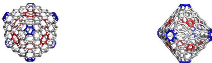
Figure 3. 3D-vue of Le(P_4(C))^2 ; v=192 ; (left) and Le(P_4(Oct))^2 ; v=192 ; (right)
