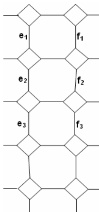
Figure 10. The Molecular Graph of TU[2,q] .
