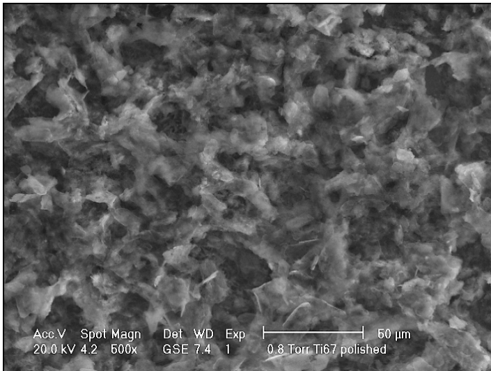
Figure 6. SEM image of the HA coating on the surface of Ti_6Al_7Nb substrate obtained with 200 W, ground and polished. Higher magnification.
