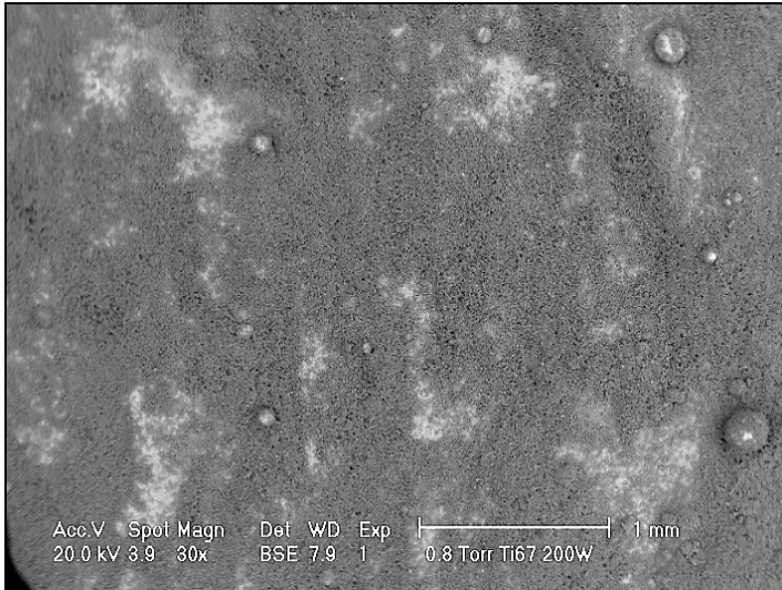
Figure 5. SEM image of the HA coating on the surface of Ti_6Al_7Nb substrate obtained with 200 W, ground and polished.
