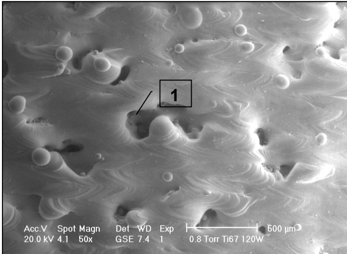
Figure 1. SEM image of the surface of the Ti_6Al_7Nb substrate processed with 120 W; 1 – pore.
