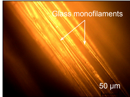
Figure 4. Non-impregnated glass fibre monofilaments
