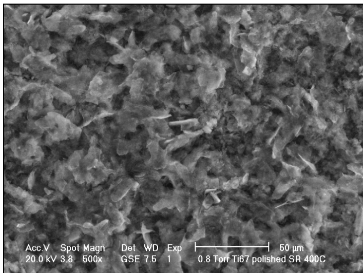
Figure 11. SEM image of the HA coating on the surface of Ti_6Al_7Nb substrate obtained with 200 W, ground and polished, then heat treated in air at 400^\circ C .
