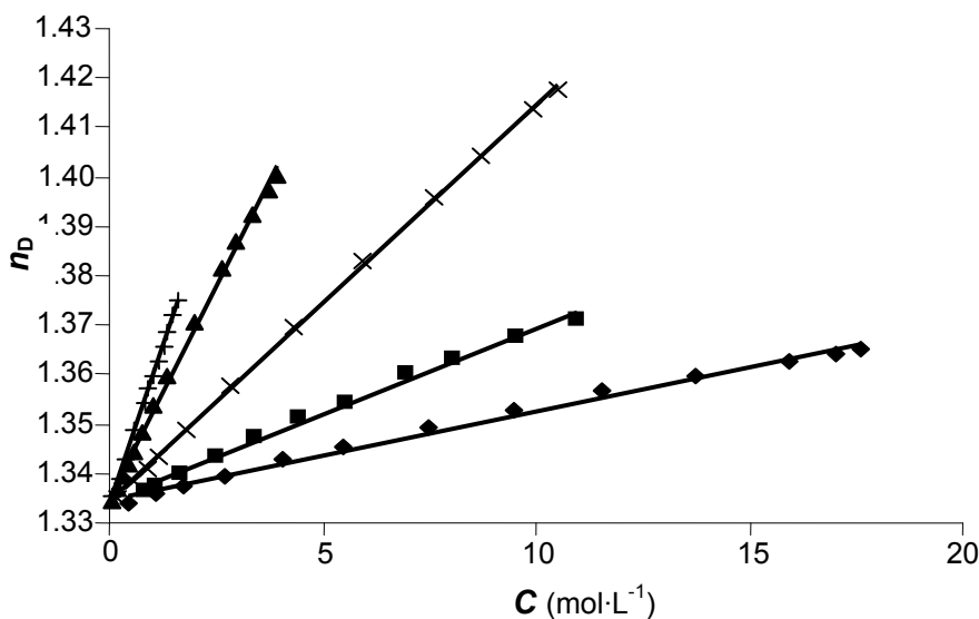
Figure 5. Refractive indices ( n_D ) plotted against molar concentration of solute ( c ) at T = 292.15 K for different aqueous solutions of: \blacklozenge , formic acid; \blacksquare , acetic acid; \blacktriangle , trichloroacetic acid; \times , lactic acid; + , citric acid.
