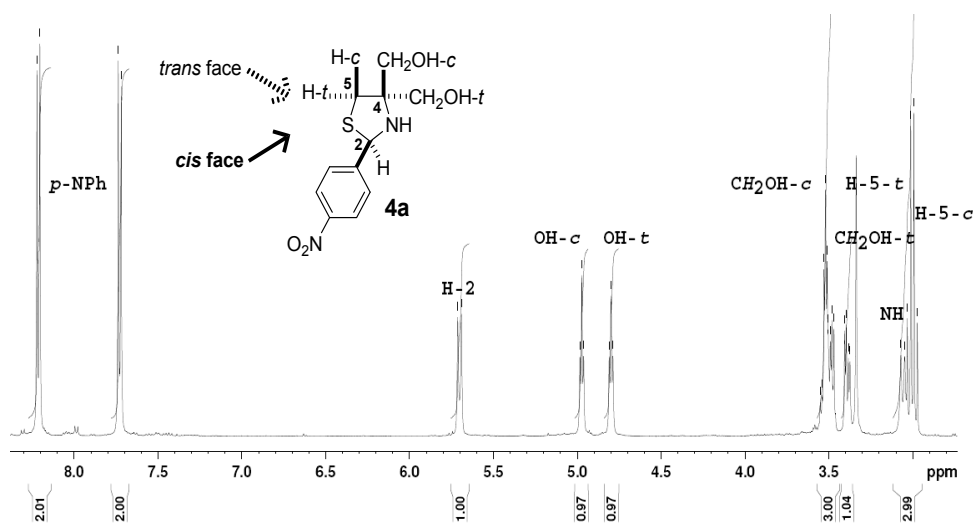
Figure 1. 1 H NMR spectrum of compound 4a (500 MHz, DMSO-d 6 , 298 K)
