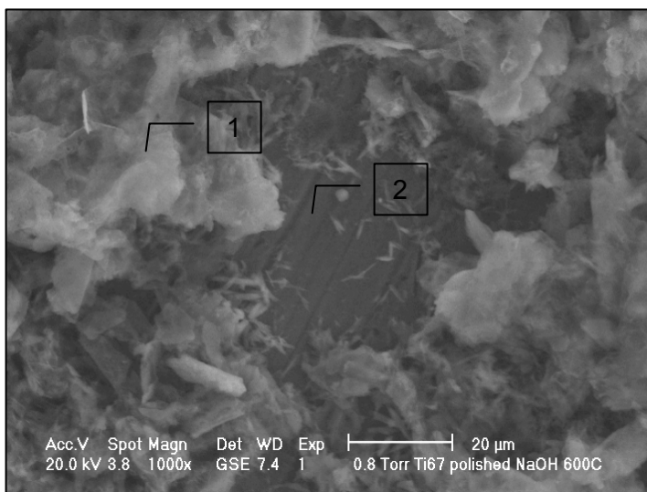
Figure 8. SEM image of the HA coating on the surface of Ti 6 Al 7 Nb substrate obtained with 200 W, ground and polished, then alkali-treated in NaOH 5M. Higher magnification. 1-HA; 2-substrate.
