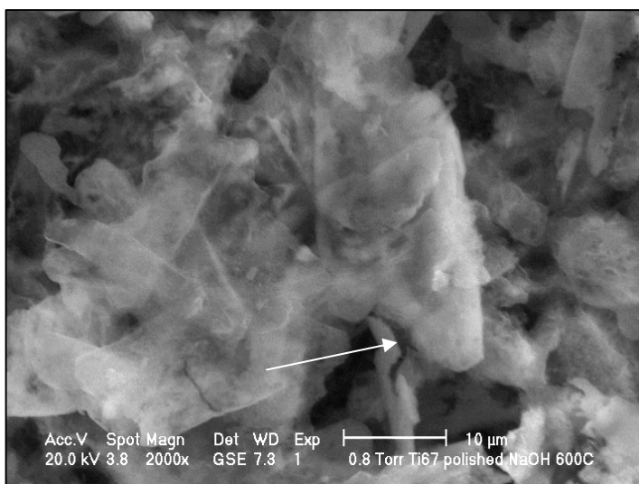
Figure 10. SEM image of the HA coating on the surface of Ti_6Al_7Nb substrate obtained with 200 W, ground and polished, then alkali treated in NaOH 5M. Micro crack indicated by the arrow.
