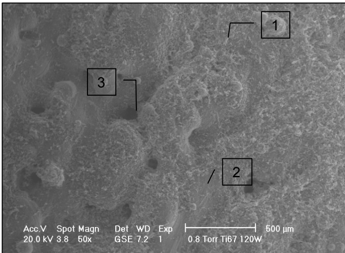
Figure 2. SEM image of the HA coated Ti_6Al_7Nb substrate processed with 120 W 1 - HA coating; 2 – substrate; 3 – pore.
