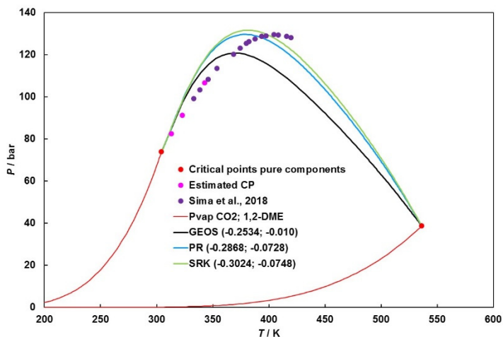
Figure 4. P – T fluid phase diagram for CO 2 (1) + 1,2-DME (2) system: (•), critical points of pure components [29]; (•), critical curve [16]; (—), vapour pressure curves; (—), critical curve calculated by GEOS ( k_{12} = -0.2534 ; l_{12} = -0.010 ); (—), critical curve calculated by SRK ( k_{12} = -0.3024 ; l_{12} = -0.0748 ); (—), critical curve calculated by PR ( k_{12} = -0.2868 ; l_{12} = -0.0728 ).
