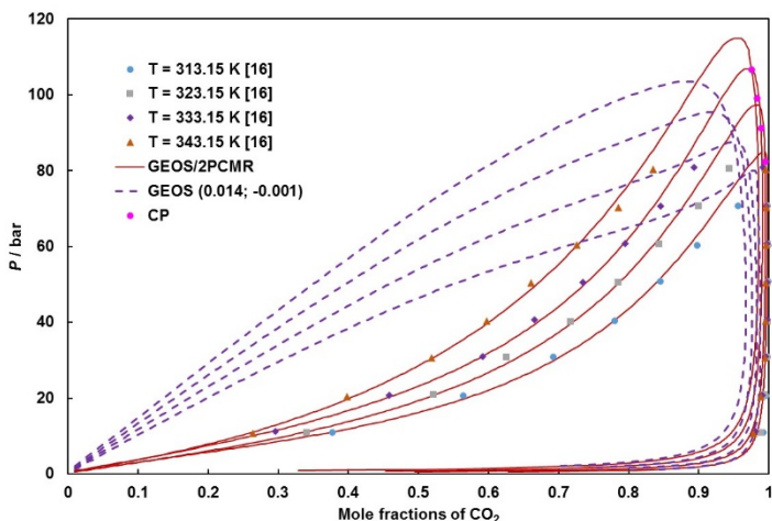
Figure 8. Comparison of correlations and predictions by GEOS for the CO_2 (1) + 1,2-DME (2) system: symbols are the experimental data [16], red solid lines are the correlations, and purple dashed lines are the semi-predictions (BIPs from Table 3 ).
